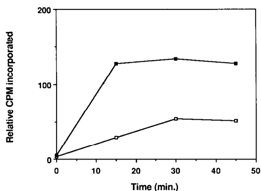
Fig. 3. [ ^3\text{H} ]Acetate incorporation into histone in isolated yeast nuclei by the endogenous histone acetyltransferase. The histone acetyltransferase assay was performed in the absence (□) or presence (■) of 2 mM spermine as described in section 2.
