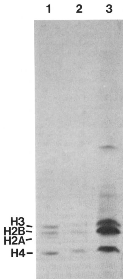
Fig. 4. Fluorogram depicting the incorporation of [ ^3\text{H} ]acetate into histone catalyzed by the endogenous yeast nuclear histone acetyltransferase. Lanes: 1, [ ^3\text{H} ]acetate-labeled chicken histone standards; 2 and 3, identical yeast samples were incubated as in fig. 3 for 20 min in the absence (2) or presence (3) of 2 mM spermine. Samples were electrophoresed on a SDS 18% polyacrylamide gel and a fluorogram prepared.
